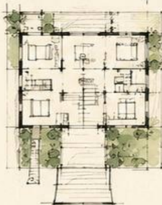
Ground Floor Plan (Concept)
